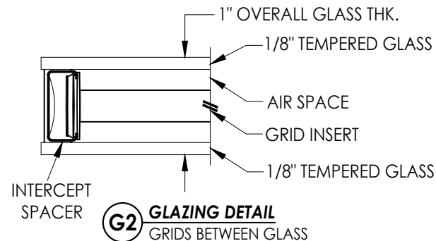
ALTERNATE GLAZING DETAILS
