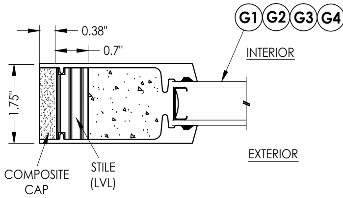
2 3 HORIZONTAL CROSS SECTION
