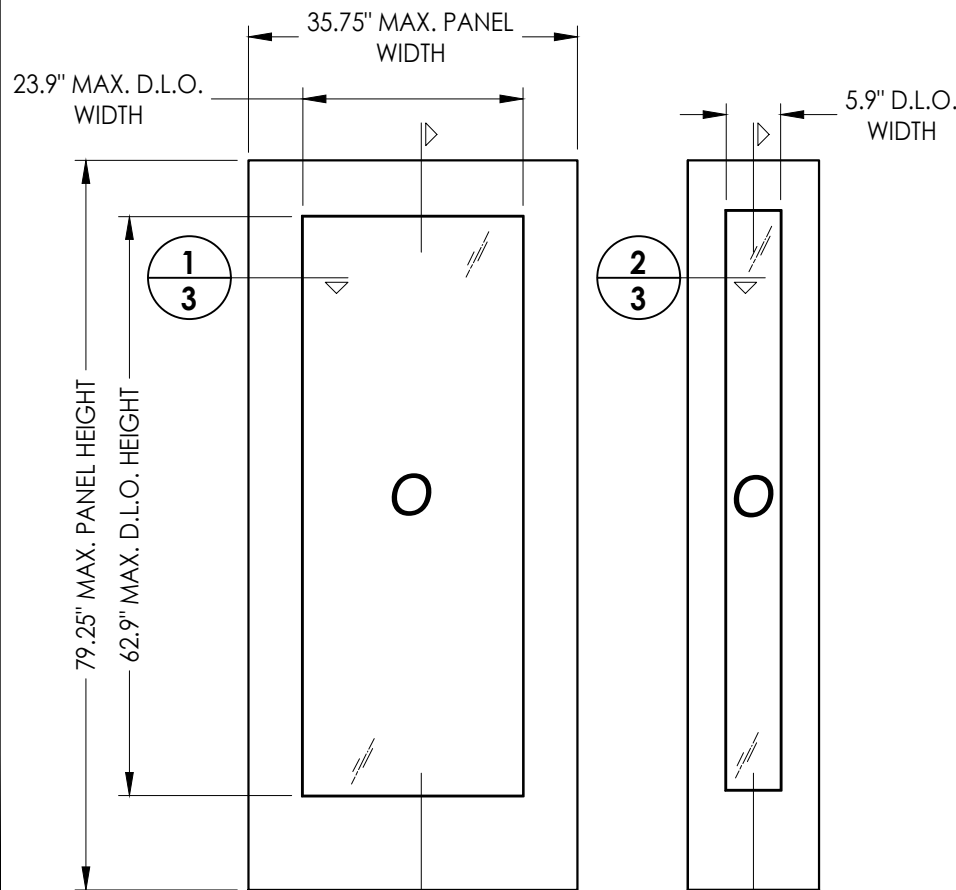
3 3 FIBERGLASS SIDELITE PANELS ODL
