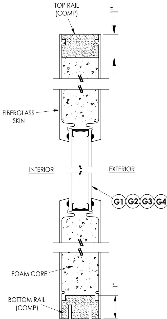
3 3 VERTICAL CROSS SECTION
