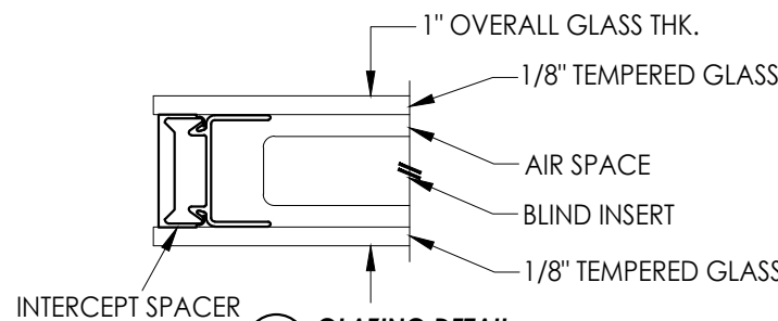
G4 GLAZING DETAIL BLINDS BETWEEN GLASS
